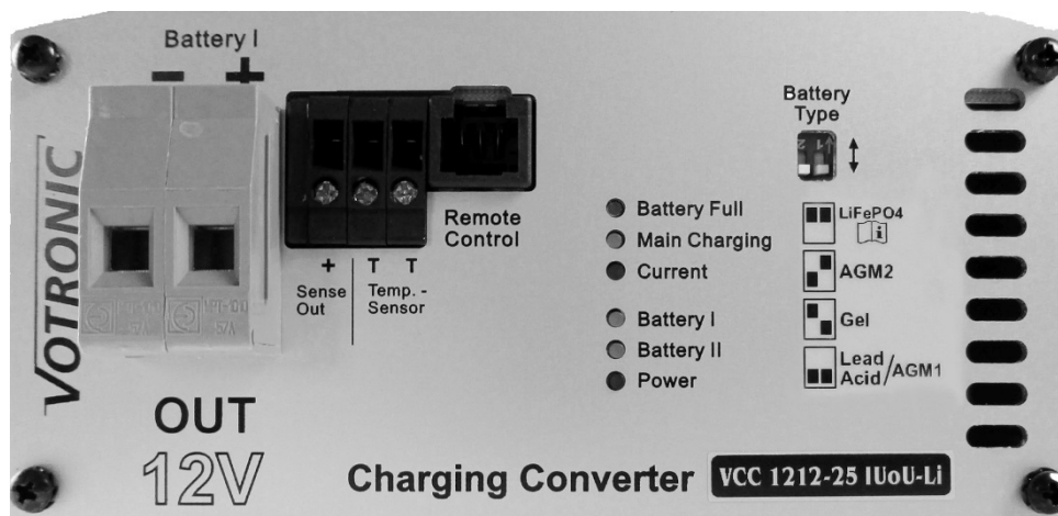
View Front Panel Output
