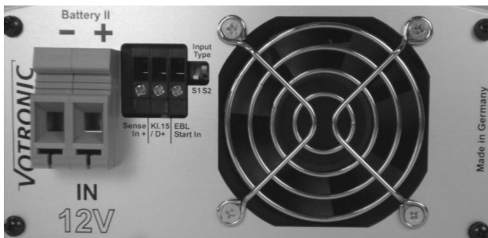
View Front Panel Input
